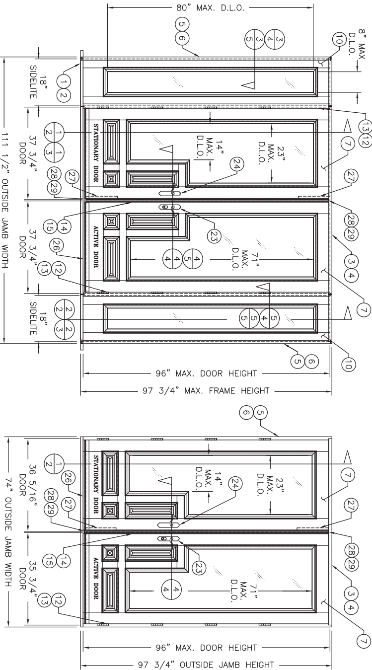
DOUBLE UNIT W/ 2 SIDELITES (OXXO) SCALE: 1/2" = 1'-0"
