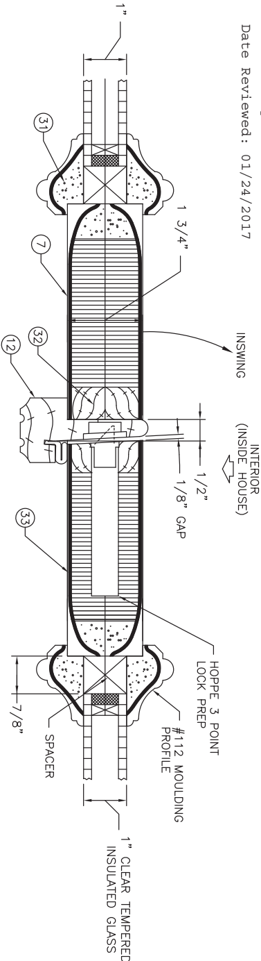
4 HORIZONTAL CROSS SECTION TYP. ASTRAGAL SCALE: 6" = 1'-0"
